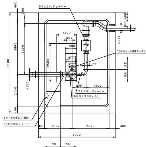
\underline{B - B}
